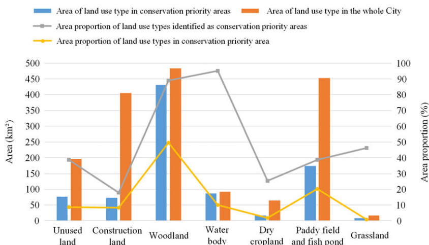
FIGURE 7 Area proportion contrast of land use types in the conservation priority area [Colour figure can be viewed at wileyonlinelibrary.com]
