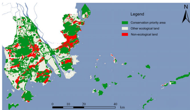
FIGURE 5 Conservation priority areas for urban ecological land in Zhuhai City [Colour figure can be viewed at wileyonlinelibrary.com ]
