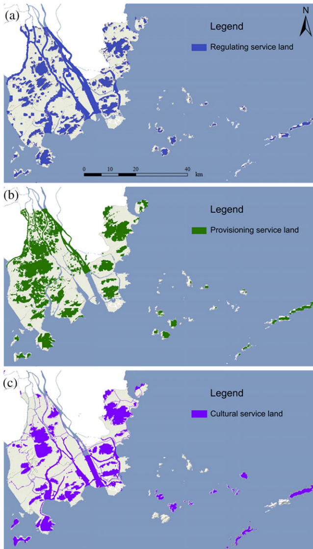
FIGURE 4 Spatial distribution of water ecosystem service land in Zhuhai City. (a) Regulating service land; (b) provisioning service land; and (c) cultural service land [Colour figure can be viewed at wileyonlinelibrary.com ]
