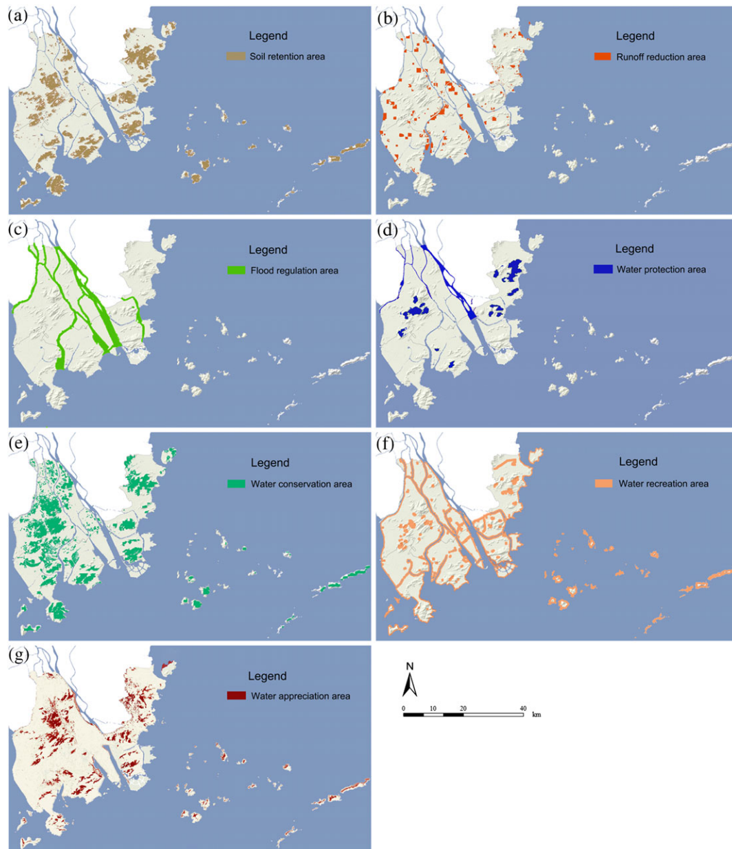
FIGURE 3 Spatial distribution of key areas for water ecosystem services in Zhuhai City. (a) Soil retention area; (b) runoff reduction area; (c) flood regulation area; (d) water protection area; (e) water conservation area; (f) water recreation area; and (g) water appreciation area [Colour figure can be viewed at wileyonlinelibrary.com ]
