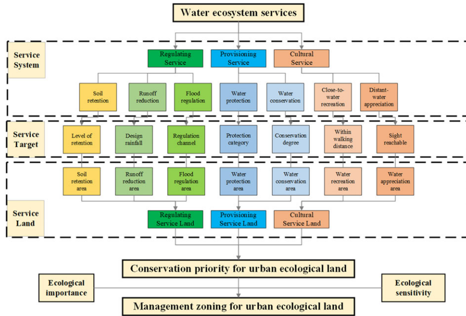
FIGURE 2 Research framework for identifying the conservation priority area and management zoning for urban ecological land [Colour figure can be viewed at wileyonlinelibrary.com ]
