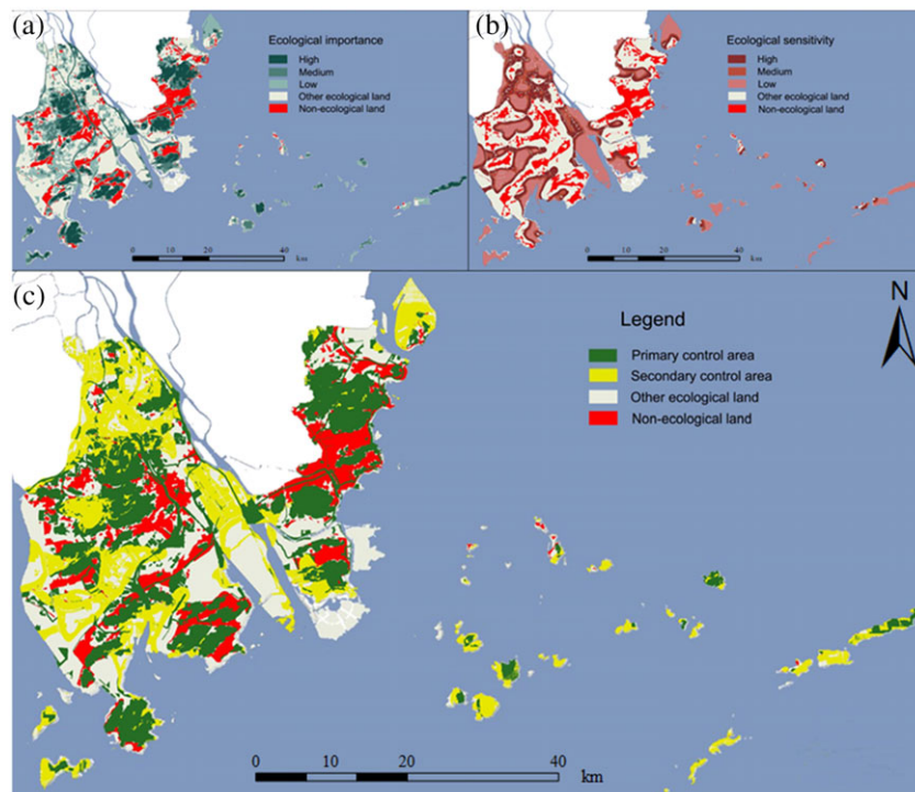
FIGURE 6 Management zoning for urban ecological land in Zhuhai City. (a) Ecological importance; (b) ecological sensitivity; and (c) management zoning [Colour figure can be viewed at wileyonlinelibrary.com]
