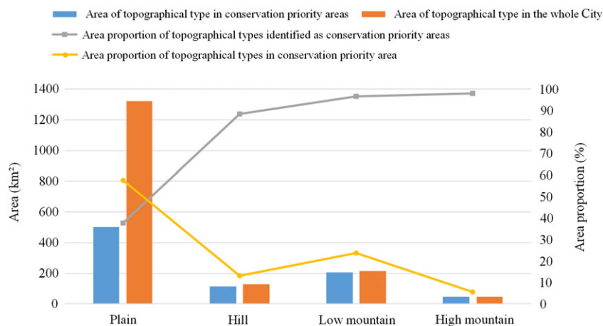
FIGURE 8 Area proportion contrast of topographical types in the conservation priority area [Colour figure can be viewed at wileyonlinelibrary.com ]
